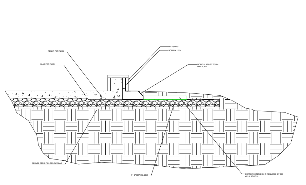
4- DRIVEWAY APPROACH
