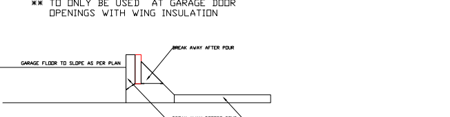
MINI FORM GARAGE DOOR OPENING END VIEW
