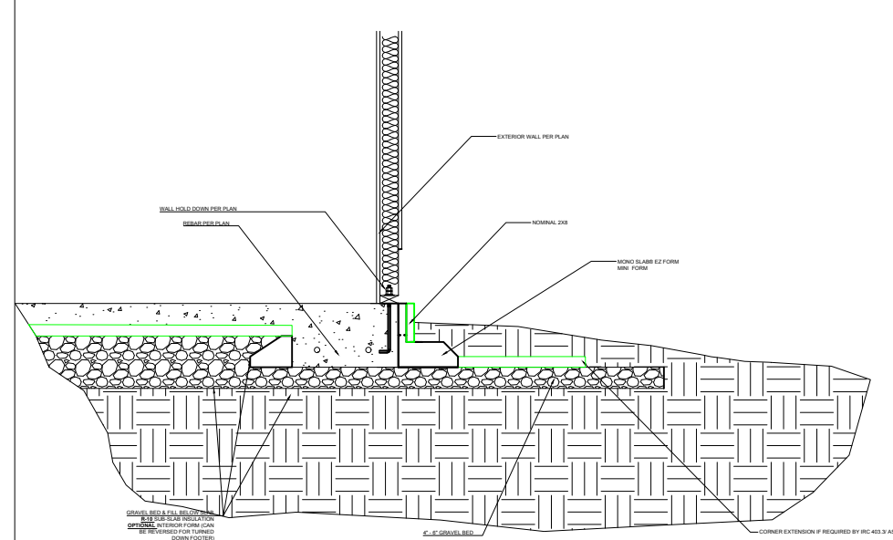
3- GARAGE STEP DOWN
