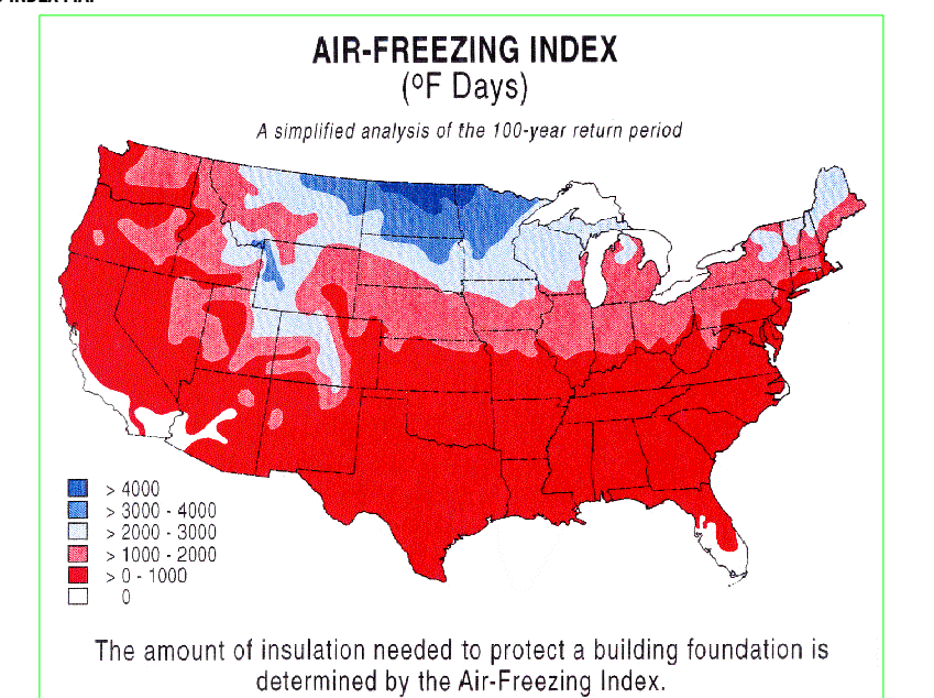
AIR FREEZING INDEX MAP
