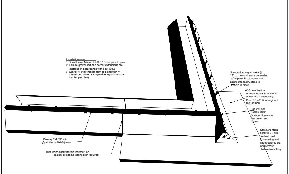
14- MONO SLAB® EZ FORM INSTALLATION
