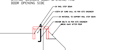
STANDARD FORM GARAGE CURB END VIEW
