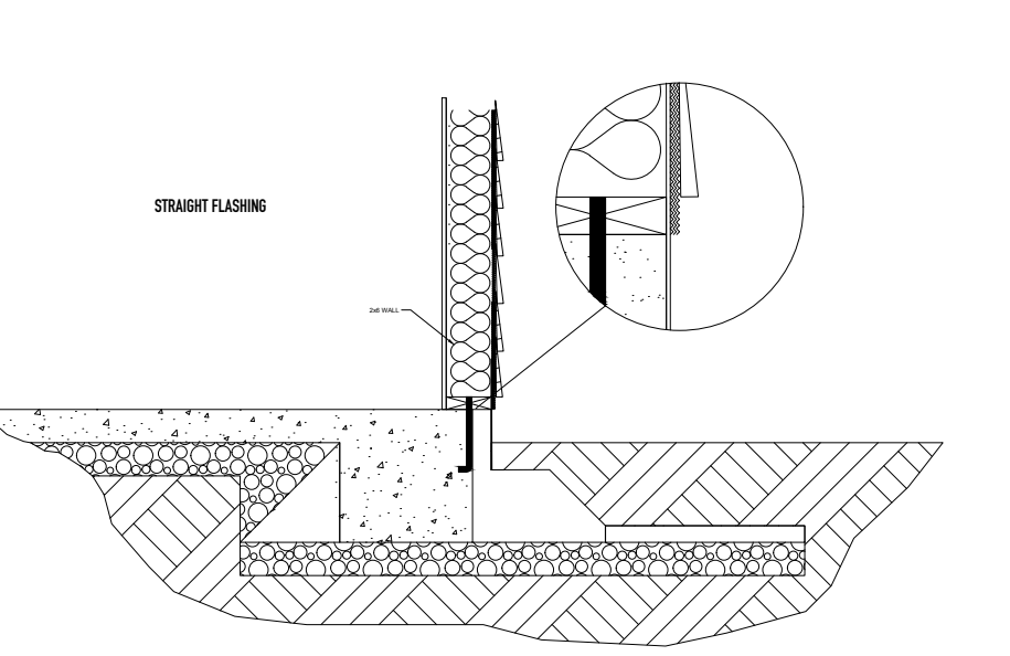
11- FLASHING
