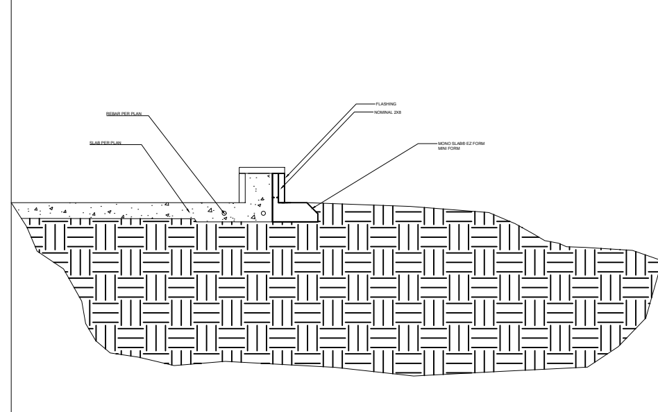
4- DRIVEWAY APPROACH
