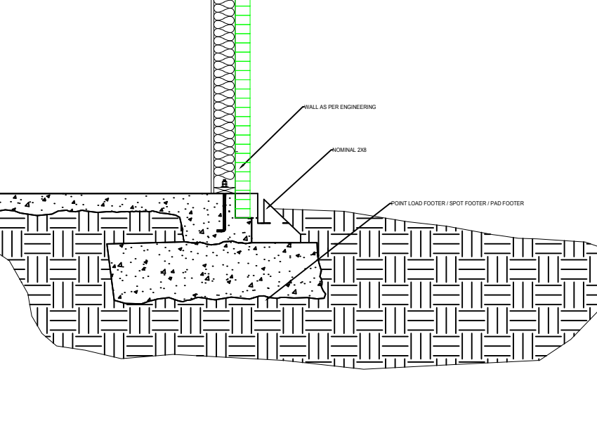
13- POST TENSION
