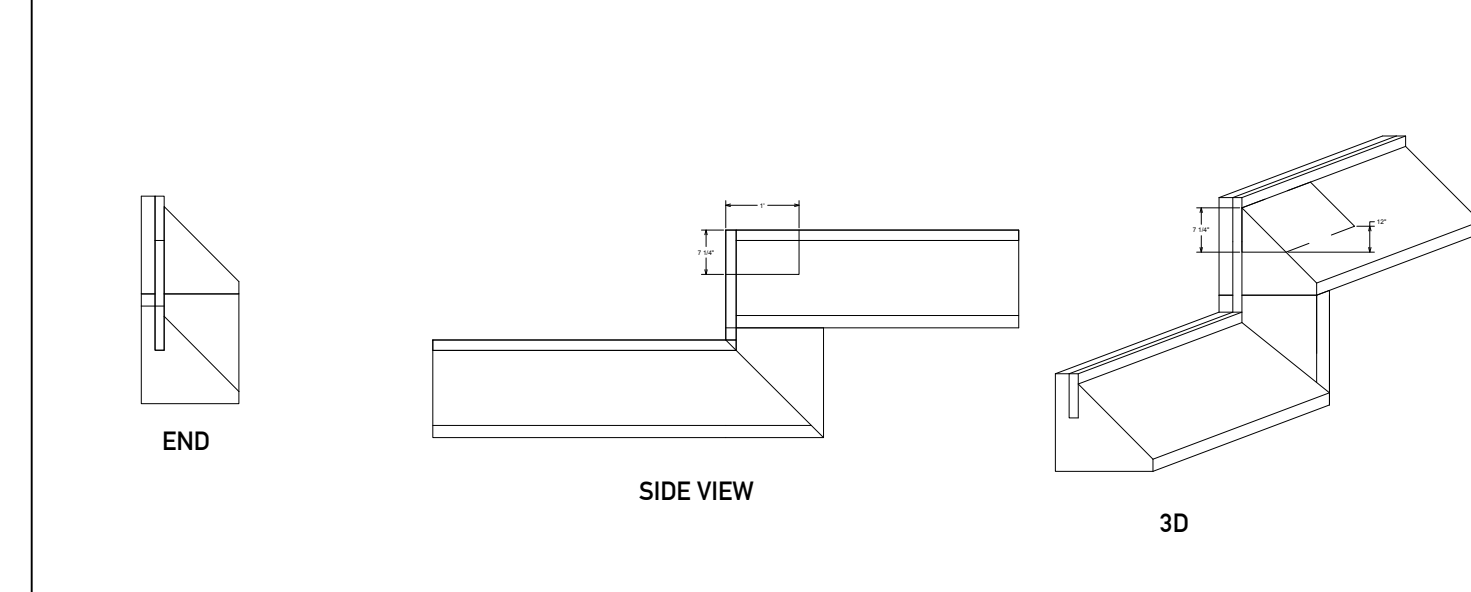
10- STEP DOWN
