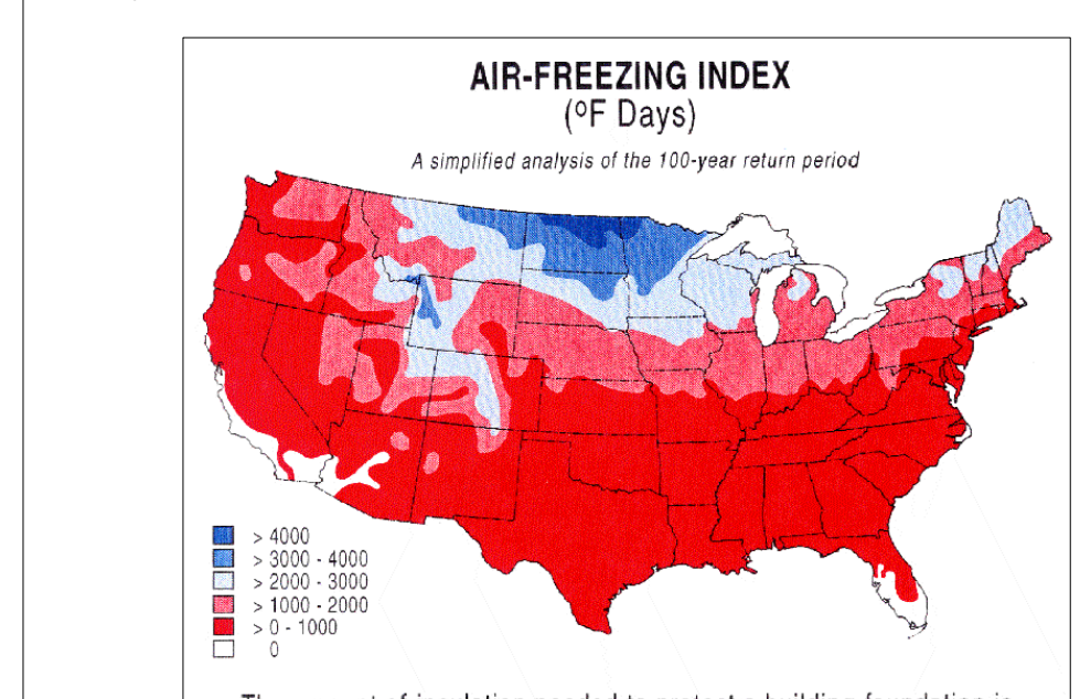
AIR FREEZING INDEX MAP
