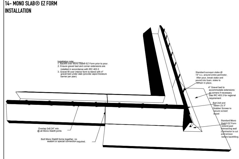
14- MONO SLAB® EZ FORM INSTALLATION
