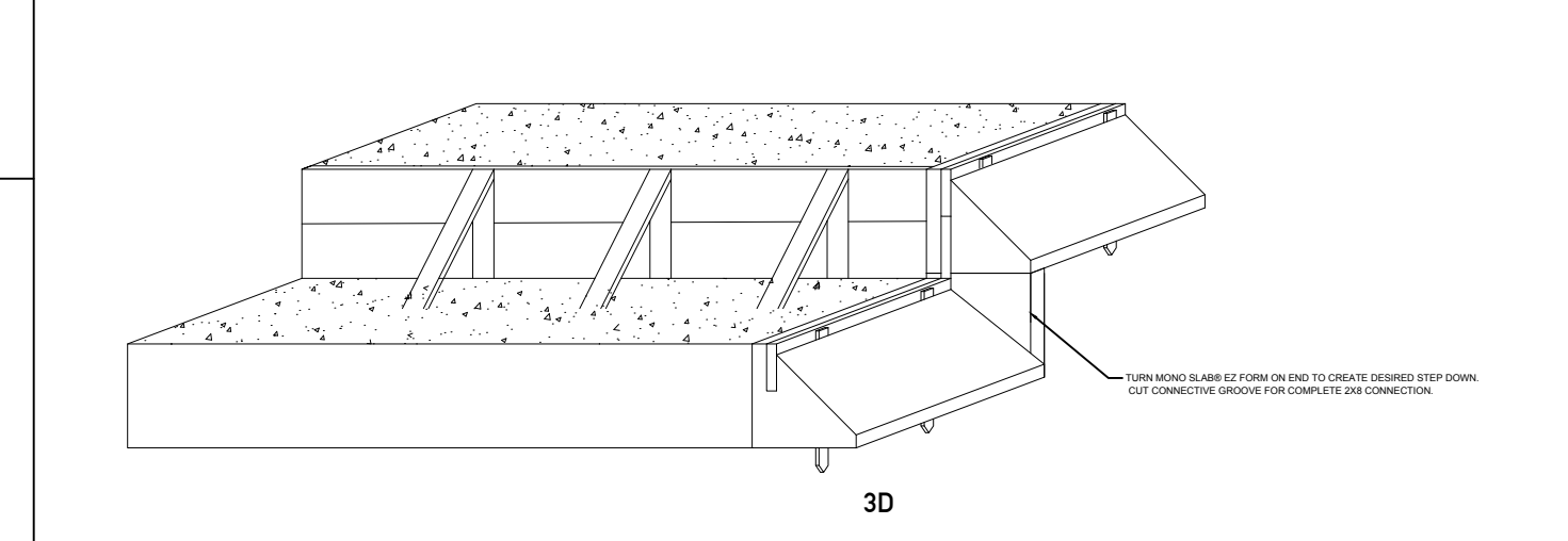
11- FLASHING
