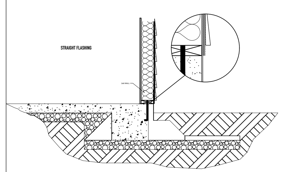
11- FLASHING
